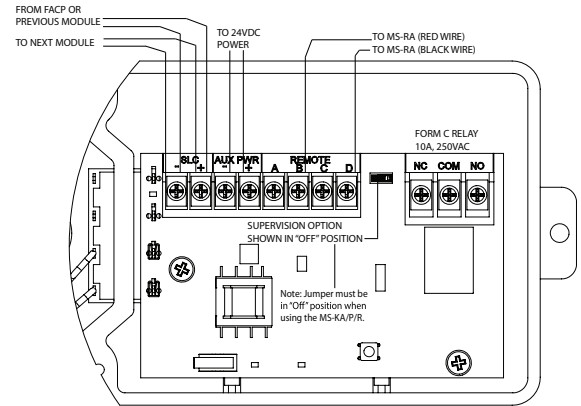
MS-KA/P/R Wiring
