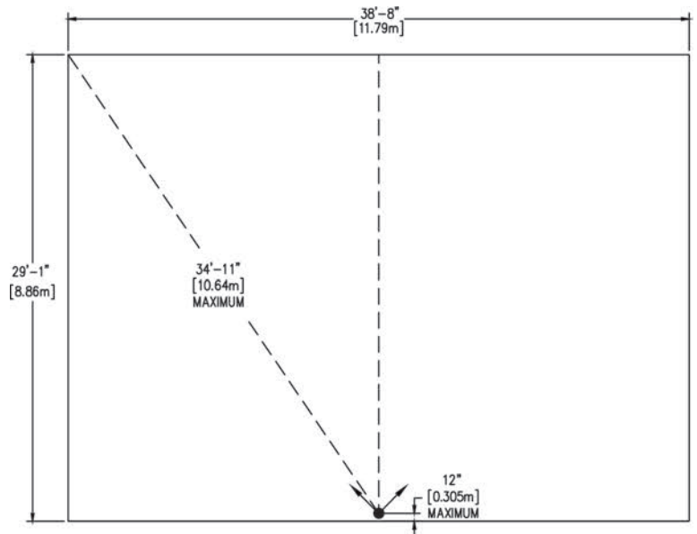
180° Sidewall Nozzle (6 Port) Arrangement
