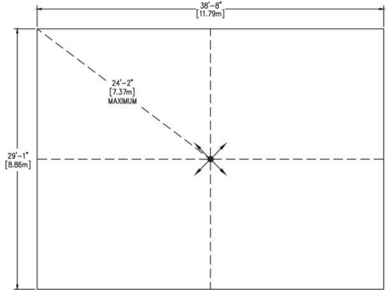
360° Radial Nozzle (8 Port) Arrangement
