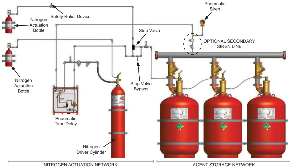
Pneumatic Arrangement
